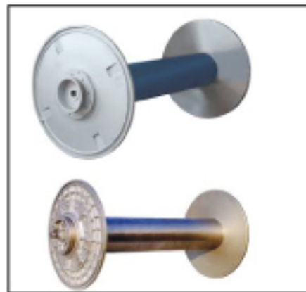
Warpor-beam
