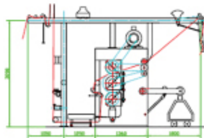
Calender machine
