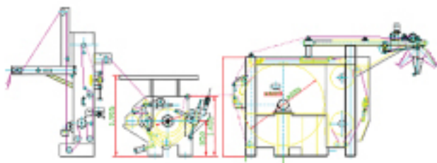
Sanforizing machine
