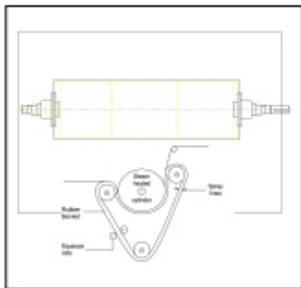
Rubber Belt Heating Cylinder
